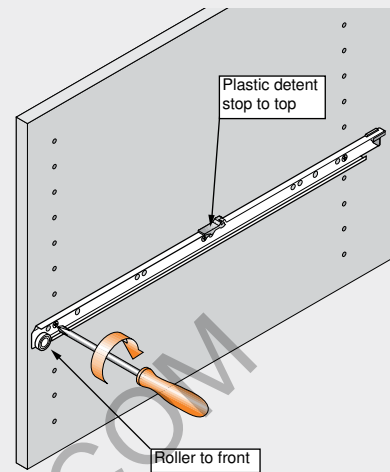
1. Mount cabinet profile to side panel
