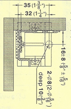
Plastic rear mounting bracket for drawer length 305(12'), 533(21')
