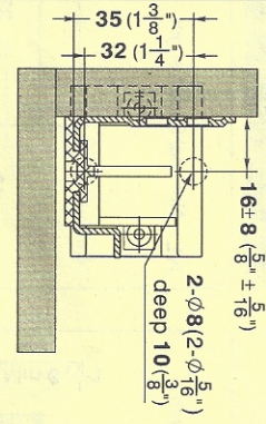
Plastic rear mounting bracket for drawer length 305(12")-533(21")
