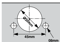
Blum hinge boring pattern
